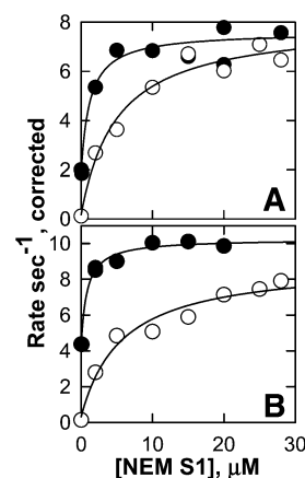
FIGURE 1: Actin-activated ATPase activity of S1 with increasing binding of activating cross-bridges, NEM-S1. The ATPase rate was corrected for S1 alone and for the hydrolysis by NEM-S1 [the residual activity of NEM-S1 was normally 0.01 \mu M ATP \text{s}^{-1} ( \mu M NEM-S1) ^{-1} ]. (A) ATPase rates in the presence of wild-type human cardiac TnT 2 reconstituted with bovine cardiac TnI and TnC. The initial rates at NEM-S1 = 0 were 2.0 \pm 0.14 and 0.15 \pm 0.028 \text{s}^{-1} ( N = 2 ) in Ca or EGTA, respectively. (B) ATP rates in the presence of the \Delta 14 TnT mutant reconstituted with bovine cardiac TnI and TnC. The initial rates were 4.5 \pm 0.24 and 0.19 \pm 0.01 \text{s}^{-1} ( N = 3 ). Symbols: solid, \text{Ca}^{2+} ; open, EGTA. Conditions: 1 mM ATP, 3 mM \text{MgCl}_2 , 10 mM MOPS, pH 7.0, 34 mM KCl, 1 mM dithiothreitol, 10 \mu M actin, 2.2 \mu M tropomyosin, and 0.2 \mu M S1.
